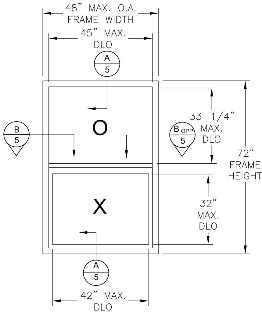
ELEVATION LAYOUT SINGLE HUNG WINDOW (INTERIOR VIEW)
