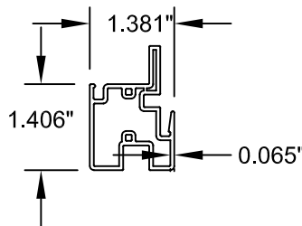
⑥ TRANSOM UPVC-606008
