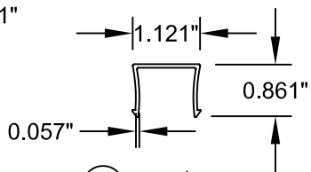
③ STOP/COVER UPVC-500124
