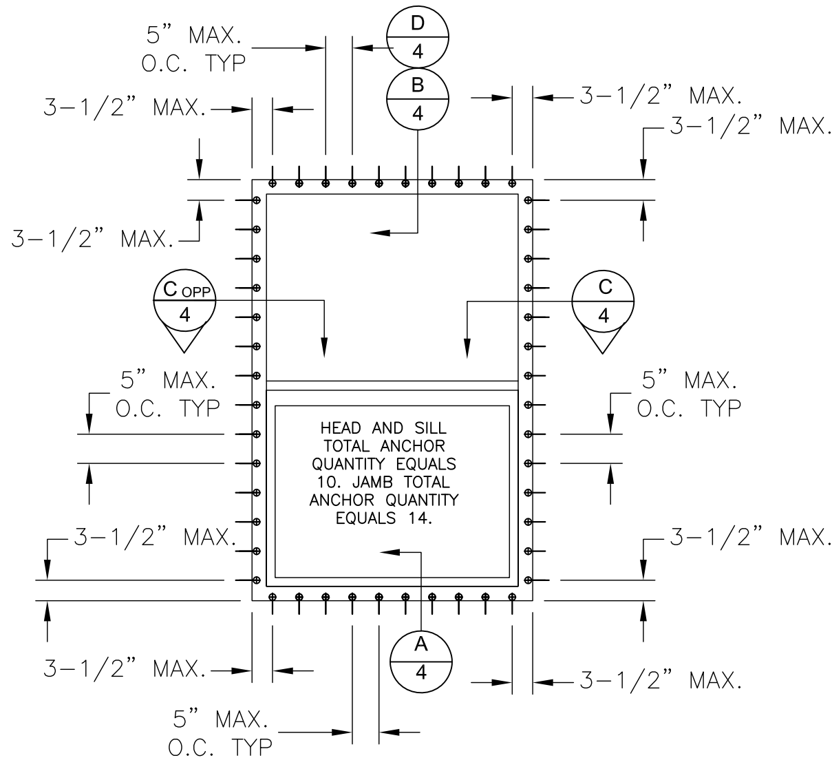
ANCHOR LAYOUT NAILING FIN 48" X 72" INSTALLATION
