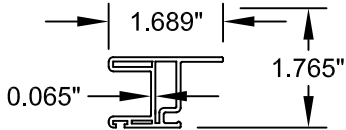
⑤ COMMON SASH UPVC-606007
