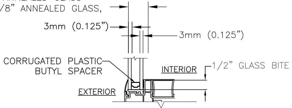
GLAZING DETAIL A
