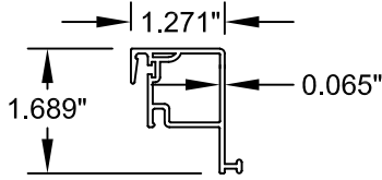
④ INTERLOCK/LIFT RAIL SASH UPVC-606005
