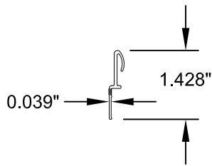
⑮ PART NO. 612496 SILL RISER-UPVC
