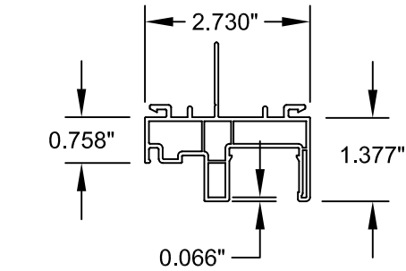
① FRAME WITH NAIL FIN EQUAL LEG UPVC-606004
