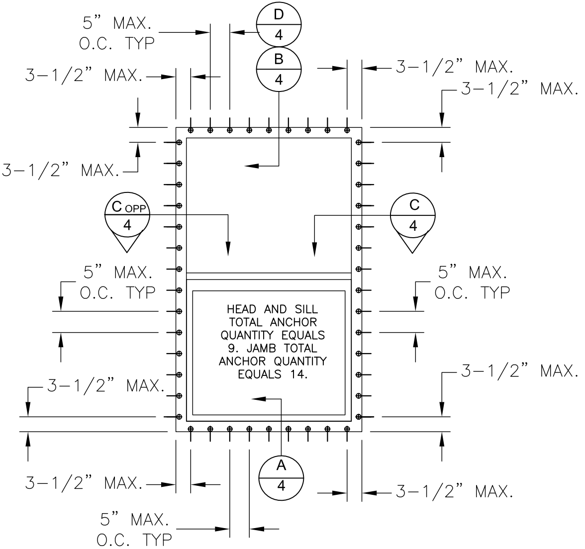
ANCHOR LAYOUT NAILING FIN 44" X 72" INSTALLATION
