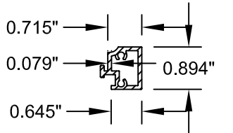
⑫ INTERLOCK LIFT RAIL ALUM. REINF.-612429
