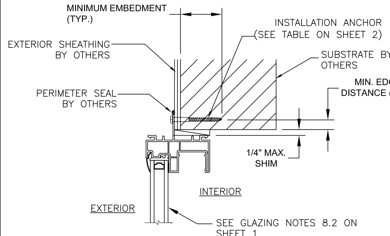
B 4 ANCHOR DETAIL NAILING FIN FRAME HEAD
