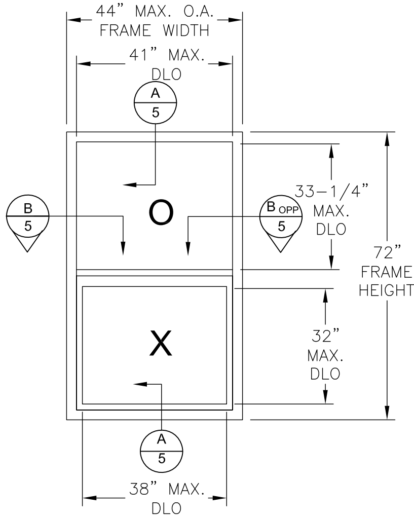
ELEVATION LAYOUT SINGLE HUNG WINDOW (INTERIOR VIEW)
